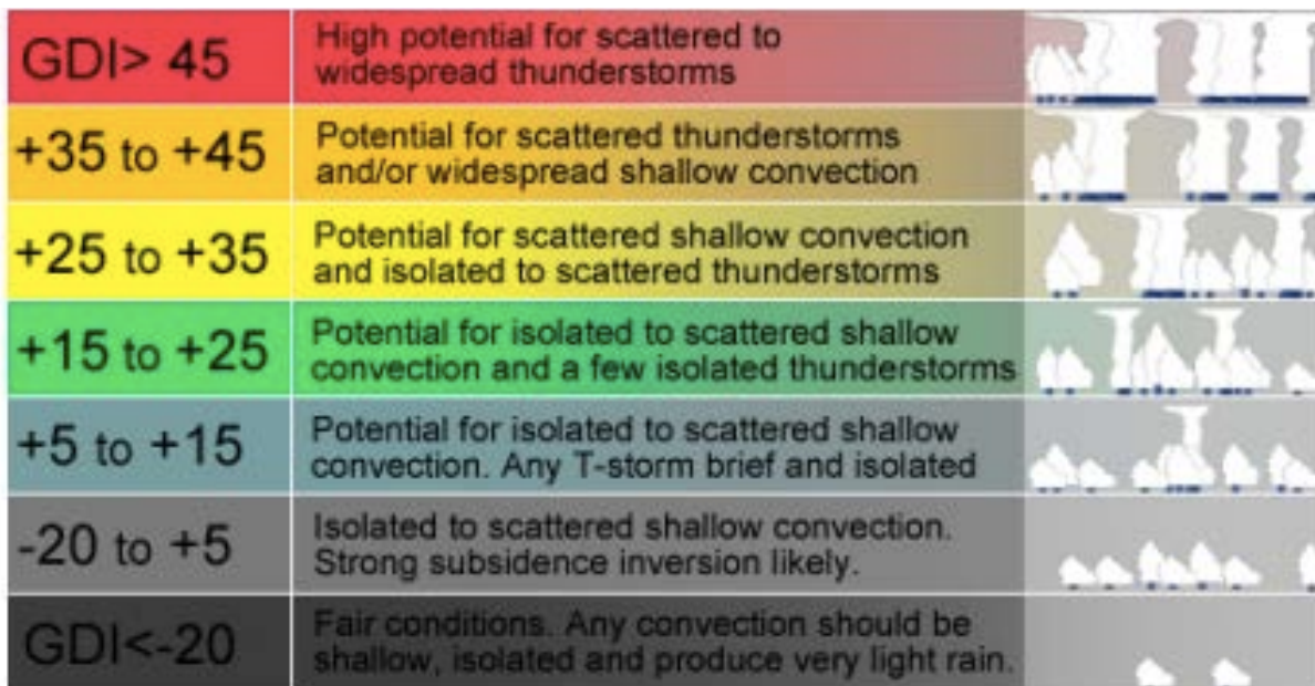
Figure 2.6: GDI values and their corresponding convective potential (Gálvez and Davison 2016).
